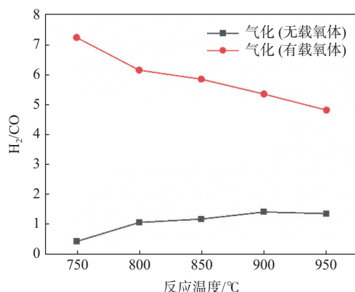
图 3 以赤泥做载氧体不同温度下蓝藻气化合成气中 H 2 /CO [40] Fig. 3 H 2 /CO in the cyanobacteria gasification syngas at different temperatures using the red mud as oxygen carriers [40]
