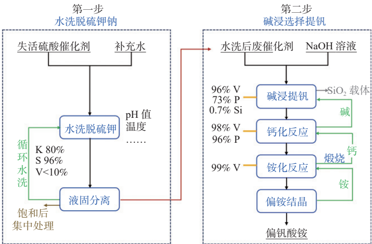
图 4 失活硫酸催化剂两步法清洁提钒工艺设计 Fig. 4 Design of vanadium extraction process by two-stage cleaning with deactivated sulfuric acid catalyst
