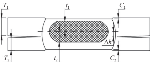
图 3 点焊接头的截面特征 Fig. 3 Schematic diagram of the cross-sectional feature of the weld
