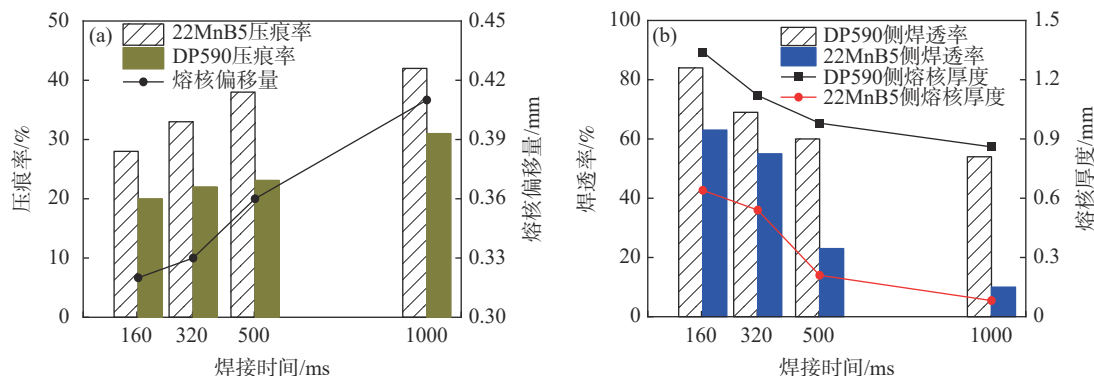
图5 焊接时间对接头截面尺寸的影响 Fig. 5 Influence of welding time on section size of joint
