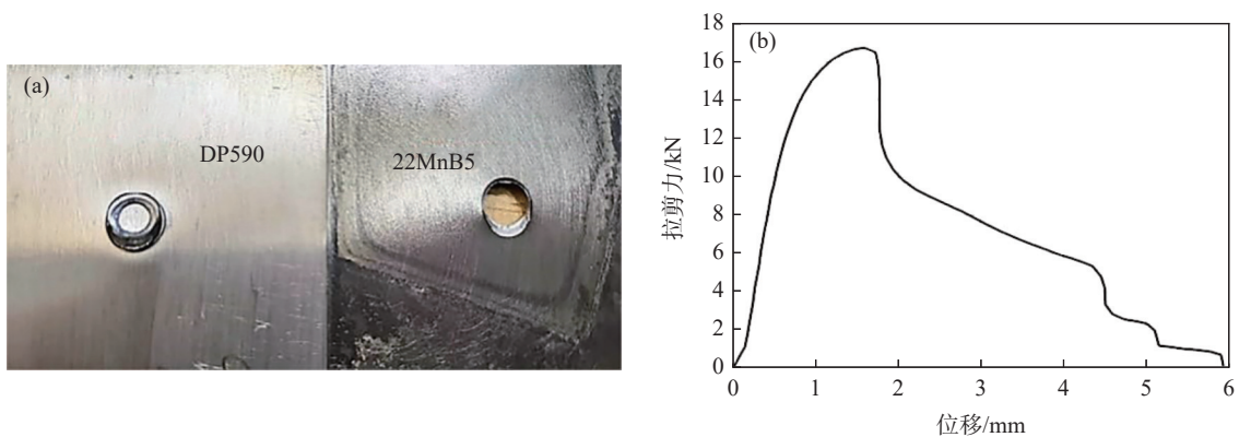
图 11 熔核拔出断裂的拉伸曲线和断口形貌 Fig. 11 Tensile curve and fracture morphology of nucleus pull-out fracture
