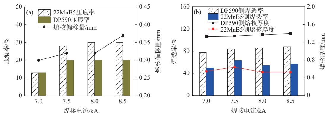
图4 焊接电流对接头截面尺寸的影响 Fig. 4 Influence of welding current on section size of joint
